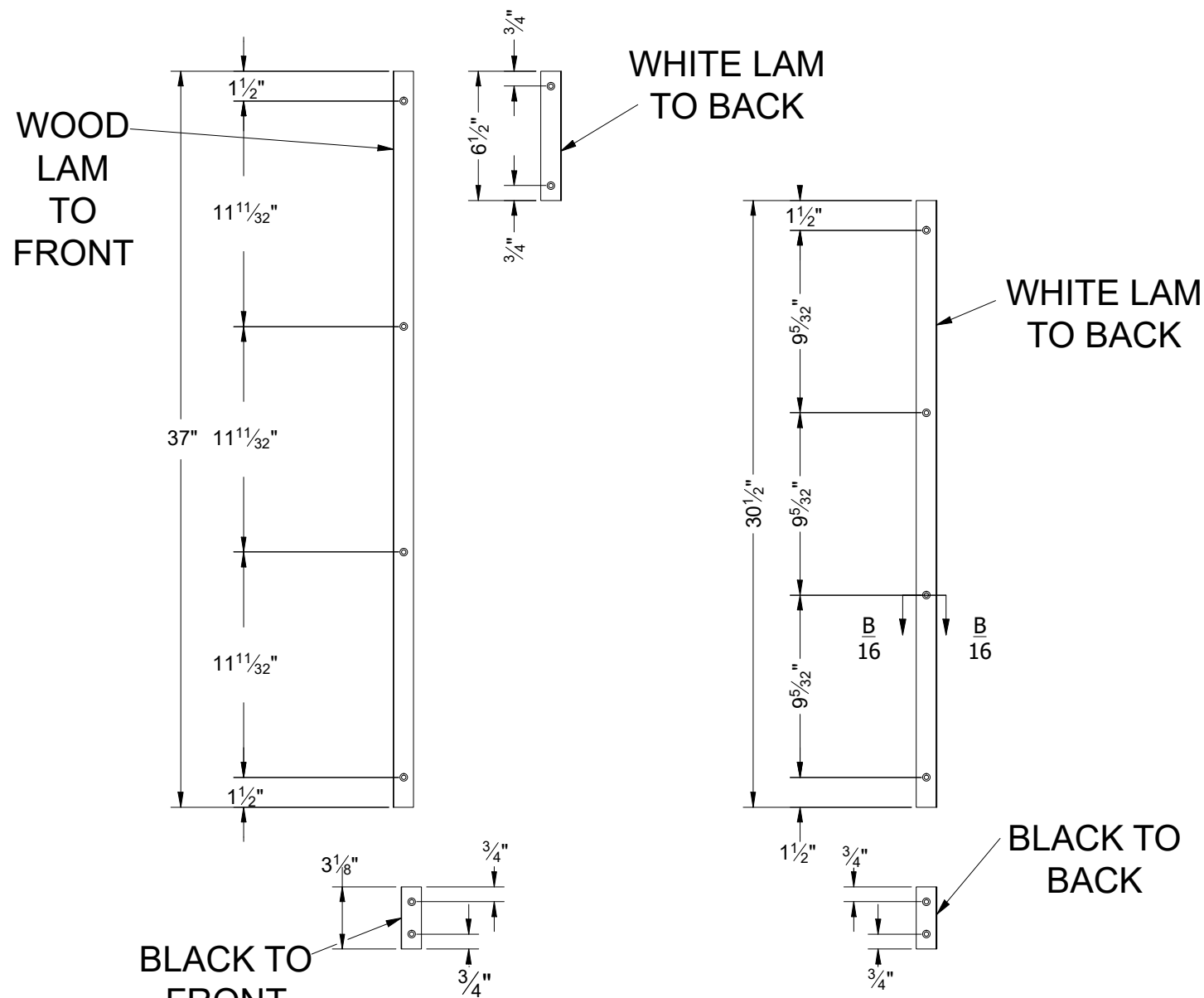
1 2C FRONT N.T.S. SERVICE DESK FILLER KIT
