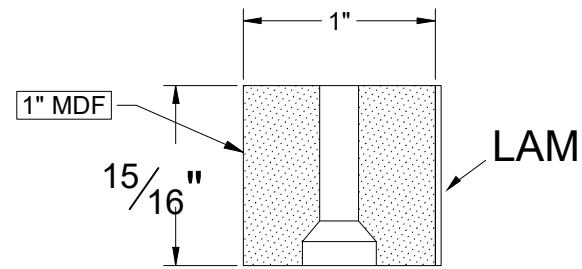
A 2C SECTION DETAIL
